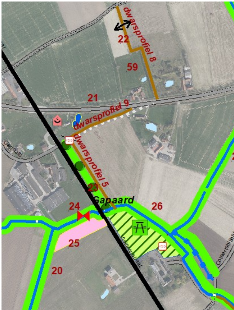
Maatregelenplan detail 5
